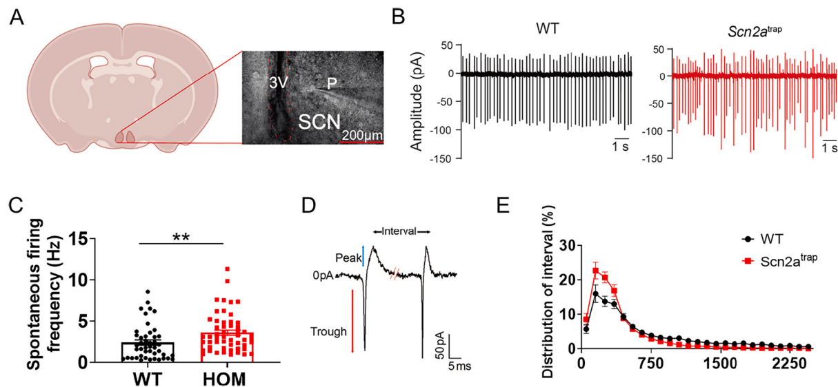
Fig. 4. Scn2a deficiency disrupts the spontaneous firing of SCN neurons. A , Illustration of the recording of SCN neurons. (P: pipette; 3 V: The third ventricle; SCN: suprachiasmatic nucleus; scale bar, 200 \mu m). B , Representative cell-attached patch traces from neurons of WT or Scn2a trap mouse. Scale bar, 1 s. C , Spontaneous AP frequencies of SCN neurons from WT and Scn2a trap mice during the light cycle (ZT2–8, WT: 6 slices from 3 mice; Scn2a trap : 6 slices from 3 mice). Scn2a deficiency resulted in an increased firing frequency. D , Illustration of two spontaneous firing events from a typical SCN neuron showing trough, peak, and interval; scale bar, 50 pA and 5 ms. E , Intervals distribution plot showing enrichment in small intervals (<500 ms) and reduction in large intervals (>500 ms) of neurons from Scn2a trap mice compared to those from WT mice. Data are presented as means \pm SEM (student's t -test; ** p < 0.01).
