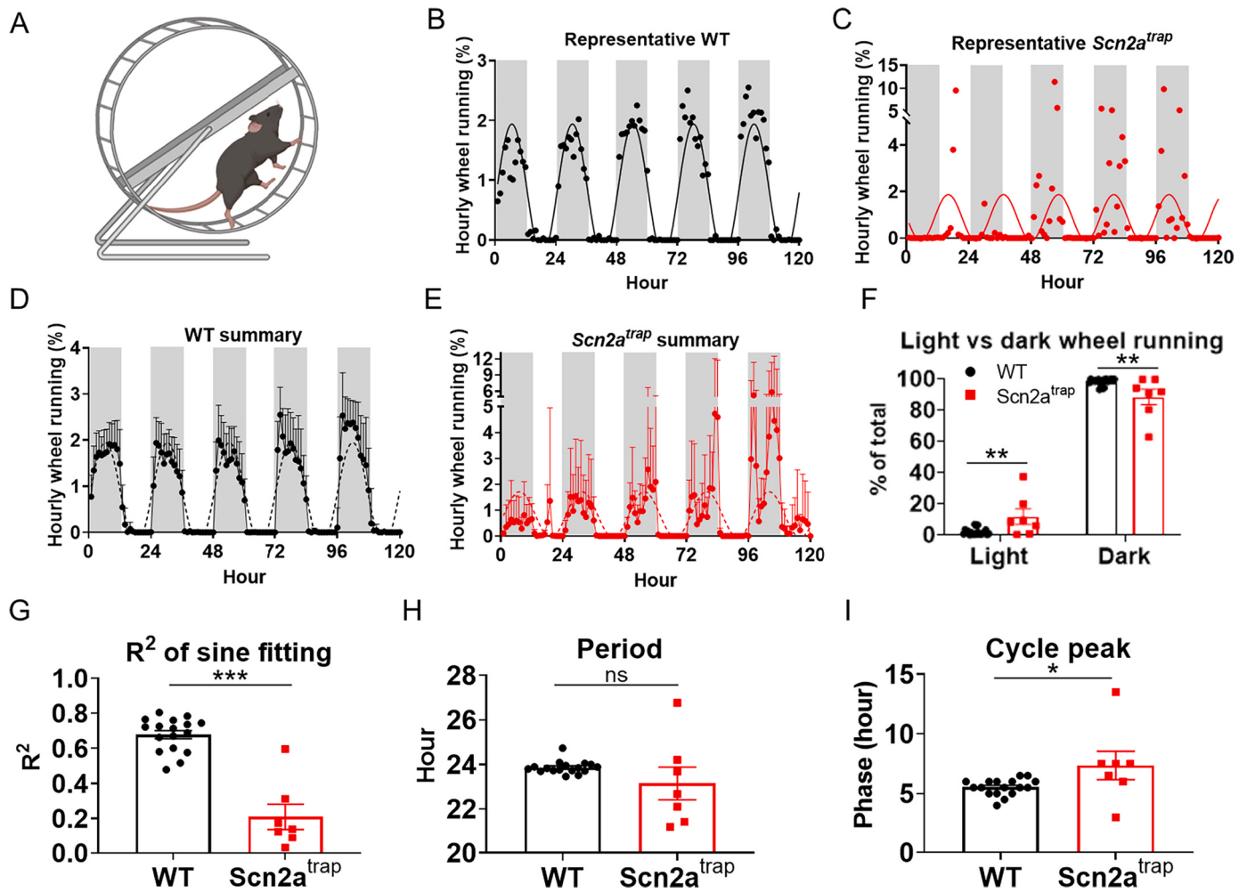
Fig. 3. Scn2a -deficient mice show impairment of wheel-running activity in light-dark conditions. A , Illustration of the wheel running assay. B-C , Representative relative wheel-running activity and sine wave fitting for WT ( B ) and Scn2a trap mice ( C ). Individual dots show the normalized activity per hour for WT and Scn2a trap mice, solid lines show the sine wave fitting of the data for WT and Scn2a trap mice. D-E , Averaged relative wheel-running activity and sine wave fitting for WT and Scn2a trap mice. Gray shading represents the dark period. Dash line shows the sine wave fitting. F , Distribution of wheel-running activity in the light and dark phases show an increased percentage in light phase wheel-running activities of Scn2a trap mice. G , the R^2 comparison of sine wave fitting for WT and Scn2a trap mice is shown. H , Period of the wheel-running activity is not different between Scn2a trap and WT mice. I , Cycle peak or phase of the wheel-running activity shows a notable difference in Scn2a trap mice compared to WT mice. No sex difference was found between males and females thus the data were combined for presentation. Data were analyzed by unpaired student's t -test and presented as means \pm SEM (* p < 0.05; ** p < 0.01; *** p < 0.001; ns p > 0.05), n = minimum of 17 WT and 7 Scn2a trap mice.
