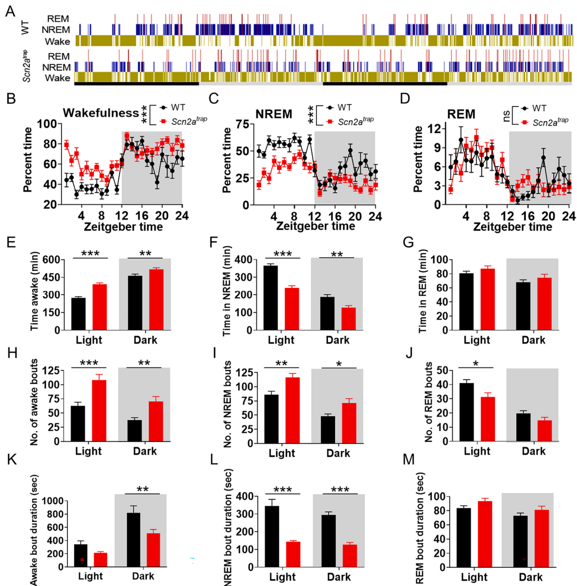
Fig. 1. Scn2a -deficient mice display abnormal sleeping patterns. A , representative 48 h long hypnograms of ultradian rhythms over the diurnal light/dark phase in freely moving WT and Scn2a -deficient ( Scn2a trap ) mice, yellow: wakefulness (Wake); blue: NREM; red: REM. B–D , Time spent in wakefulness ( B ), NREM ( C ), and REM ( D ) states showed as a percentage of recording time per hour. E–G , Time spent in wakefulness ( E ), NREM ( F ), and REM ( G ) in light (left) and dark (right) phases between WT and Scn2a trap mice, respectively. H–J , Number of bouts in wakefulness ( H ), NREM ( I ), and REM ( J ) in light (left) and dark (right) phases between WT and Scn2a trap mice, respectively. K–M , Duration of bouts in wakefulness ( K ), NREM ( L ), and REM ( M ) in light (left) and dark (right) phases between WT and Scn2a trap mice, respectively. No sex difference was found between males and females thus the data were combined for presentation. Data were analyzed by two-way ANOVA with Bonferroni's multiple comparisons test. All data are presented as means \pm SEM (* p < 0.05; ** p < 0.01; *** p < 0.001), n = minimum of 9 WT and 11 Scn2a trap mice.
