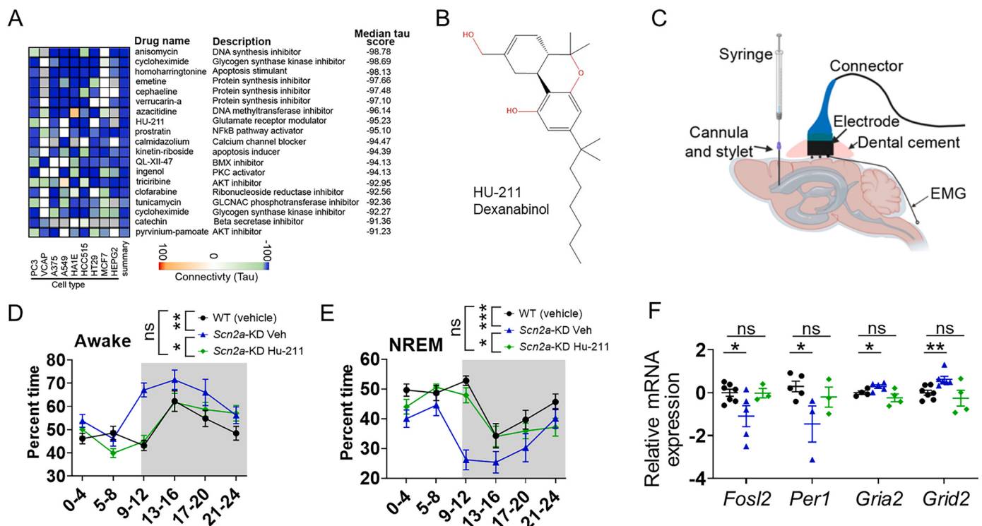
Fig. 6. Putative glutamate receptor modulator dexamabinol (HU-211) partially reverses the sleep disturbance phenotypes. A , Connectivity map analysis of the top 100 DEGs identified by RNA-sequencing predicts the compounds that may reverse the altered transcriptome. B , Structure of the HU-211. C , Schematic for the intraventricular injection to administer HU-211 and implantation of EEG electrodes on the skull of the mice. D , Time spent every four hours for the wakefulness showing that HU-211 was able to partially reduce wakefulness in Scn2a -KD mice towards the WT level. E , Time spent in every four hours for the NREM sleep showing that HU-211 was able to partially increase NREM sleep of Scn2a -KD mice towards the WT level. Repeated measures two-way ANOVA with post-hoc pairwise comparisons using Bonferroni's multiple comparisons test with n = minimum of 13 WT (vehicle), 11 Scn2a -KD (vehicle), and 10 Scn2a -KD (HU-211). F , qPCR assay of the mRNA expression patterns of Fos12 , Per1 , Gria2 , and Grid2 genes in hypothalamus samples of Scn2a -KD mice treated with vehicle, Scn2a -KD mice treated with HU-211, and WT mice treated with vehicle (student's t -test). Black: WT control with vehicle injection; Blue: Scn2a -KD mice with vehicle injection; Green: Scn2a -KD mice with HU-211 injection. Data are presented as means \pm SEM (* p < 0.05 ; ** p < 0.01 ; *** p < 0.001 ; ns p > 0.05 ).
