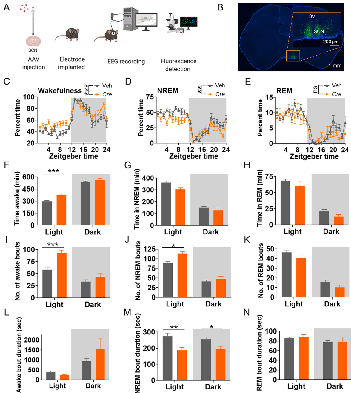
Fig. 2. Cre recombinase-mediated Scn2a deficiency in SCN containing region produces sleep disturbance. A , Scheme of the conditional knockout strategy of Scn2a and EEG recording procedure of the mice. B , brain slice imaging of Cre-virus injection into the SCN containing region and enlarged imaged showing SCN region (3 V: third ventricle). C–E , Time spent in wakefulness ( C ), NREM ( D ), and REM ( E ) showed as a percentage of recording time per hour. F–H , Time spent in wakefulness ( F ), NREM ( G ), and REM ( H ) of tm1c mice with Cre-virus (Cre) or control virus (Veh) injection. I–K , Number of bouts in wakefulness ( I ), NREM ( J ), and REM ( K ) of tm1c mice with Cre-virus (Cre) or control virus (Veh) injection. L–N , Duration of bouts in wakefulness ( L ), NREM ( M ), and REM ( N ) of tm1c mice with Cre-virus (Cre) or control virus (Veh) injection. Data were analyzed by two-way ANOVA with post-hoc comparisons using Bonferroni's correction. Veh: vehicle. Cre: mouse with Cre virus injection in SCN containing region to achieve brain region-specific Scn2a deficiency. Data are presented as means \pm SEM (* p < 0.05; ** p < 0.01; *** p < 0.001), n = minimum of 12 vehicle and 14 Cre mice.
