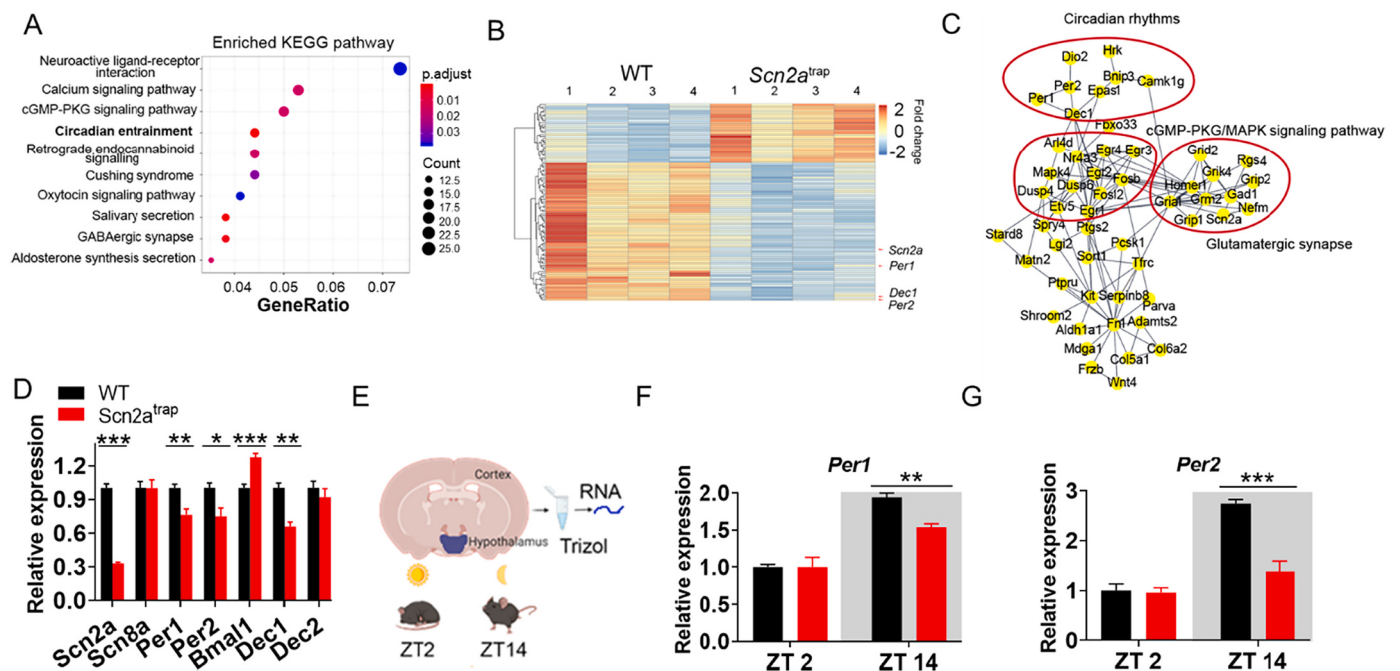
Fig. 5. Scn2a deficiency results in an altered circadian entrainment pathway and change of core clock genes expressions. A , Kyoto Encyclopedia of Genes and Genomes (KEGG) pathway enrichment analysis showing altered pathways based on differentially expressed genes (DEG) between WT and Scn2a trap groups. Note that the circadian entrainment pathway is ranked fourth. B , Heatmap of the top 100 DEG between WT vs Scn2a trap groups (ranking by q-value), showing Scn2a , Per1 , Per2 , and Dec1 as highly downregulated genes. The heatmap also shows a significantly different expression signature between WT and Scn2a trap mice. C , Protein-protein interaction map of the DEG between WT and Scn2a trap , showing circadian rhythms, cGMP/PKG/MAPK signaling pathway, and glutamatergic synapse clusters. D , qPCR analysis of relative mRNA expression of Scn2a , Scn8a , Per1 , Per2 , Bmal1 , Dec1 , and Dec2 from both WT and Scn2a trap mice. E , Illustration of dissected brain regions for qPCR analysis at two different time points. F , The Per1 mRNA expression at ZT2 and ZT14 in the SCN-containing hypothalamus of WT and Scn2a -deficient mice. G , The Per2 mRNA expression at ZT2 and ZT14 in the SCN-containing hypothalamus of WT and Scn2a -deficient mice. Unpaired student's t -test. Data are presented as means \pm SEM (* p < 0.05; ** p < 0.01; *** p < 0.001), n = minimum of 4 WT and 3 Scn2a trap mice.
